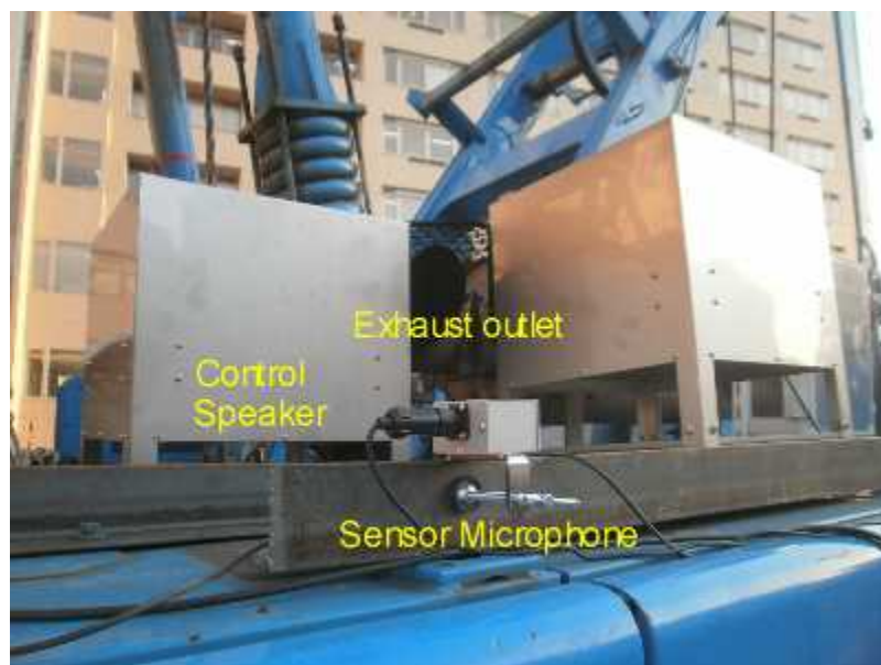
ANC (Active Noise Control) for the engine exhaust noise.
